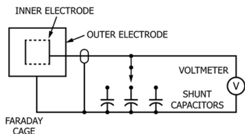
FIG. 2 Schematic Diagram
